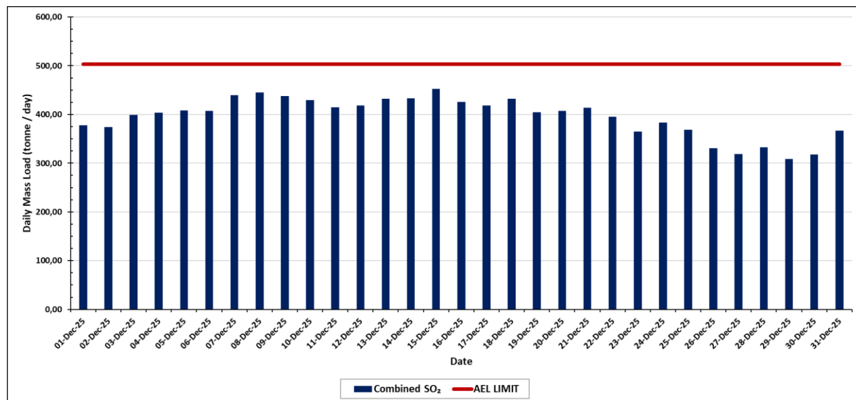
Figure 6: SO daily average SO 2 load-based limit for the period 1 st December 2025 to 31 st December 2025
