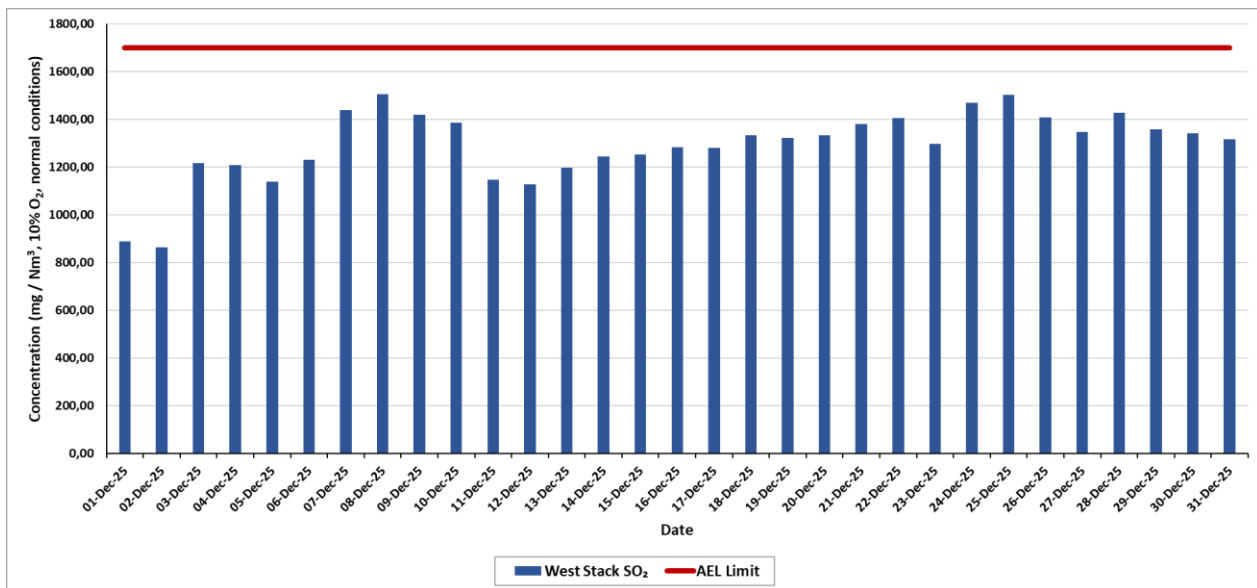
Figure 5: SO measured daily average SO 2 emissions in the West stack at 10% O 2 correction for the period 1 st December 2025 to 31 st December 2025
