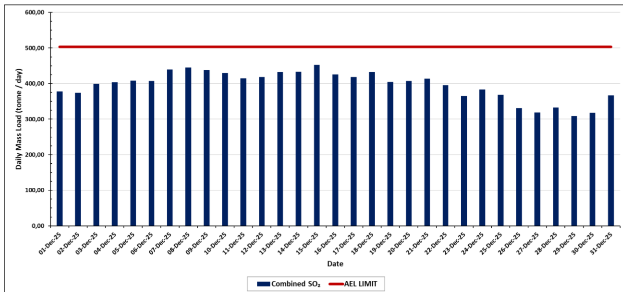
Figure iv: SO daily average SO 2 load-based limit for the period 1 st December to 31 st December 2025
