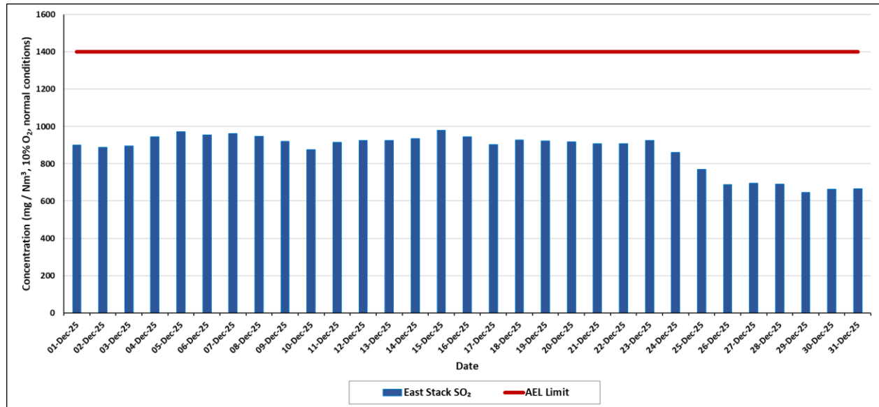
Figure 4: SO measured daily average SO 2 emissions in the East stack at 10% O 2 correction for the period 1 st December 2025 to 31 st December 2025
